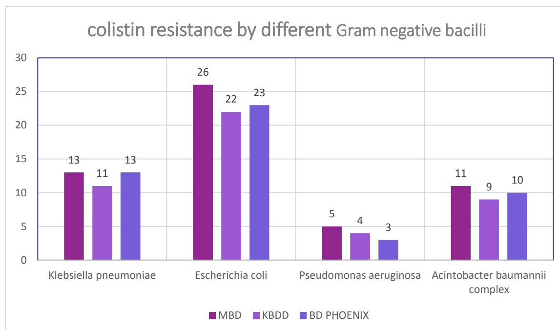
Figure 2. Colistin resistance shown by different gram-negative bacilli MBD: Broth Microdilution method, KBDD: Kirby-Bauer disk diffusion
