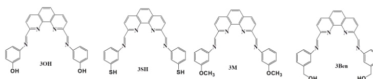
Schem3- Chemical structure of the new Schiff base derivatives
