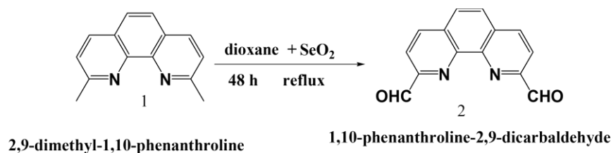
Scheme 2- Preparation of 1,10-phenanthroline-2,9-dicarbaldehyde
